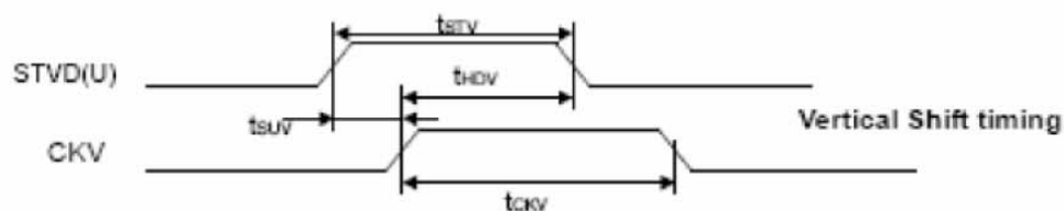
Vertical timing
